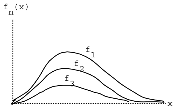
Figure 6: These f_n converge to 0 uniformly (and hence pointwise).
