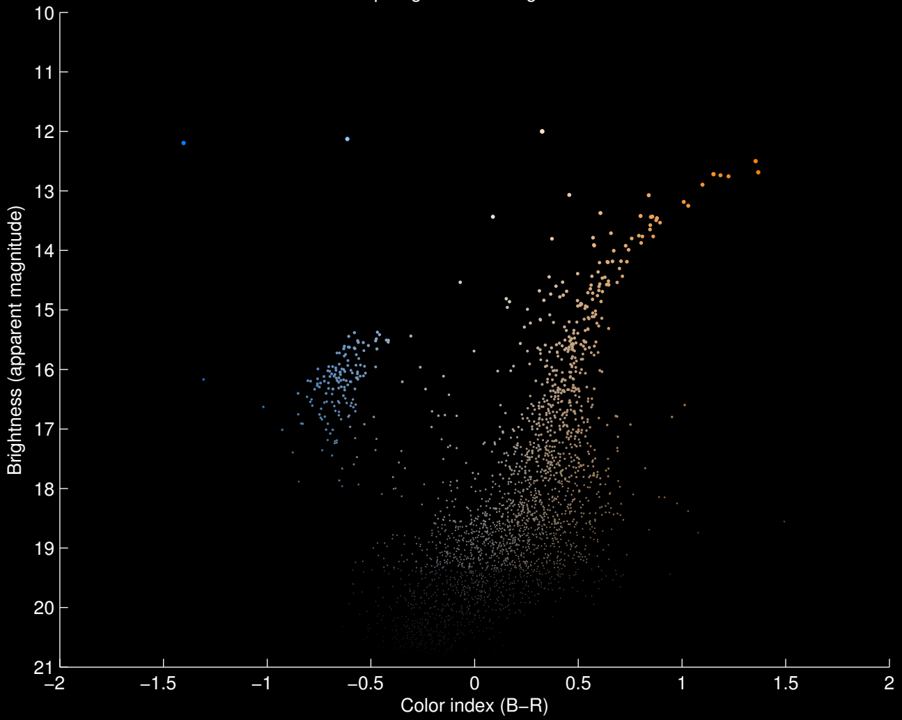
Hertzprung–Russell Diagram for M12
