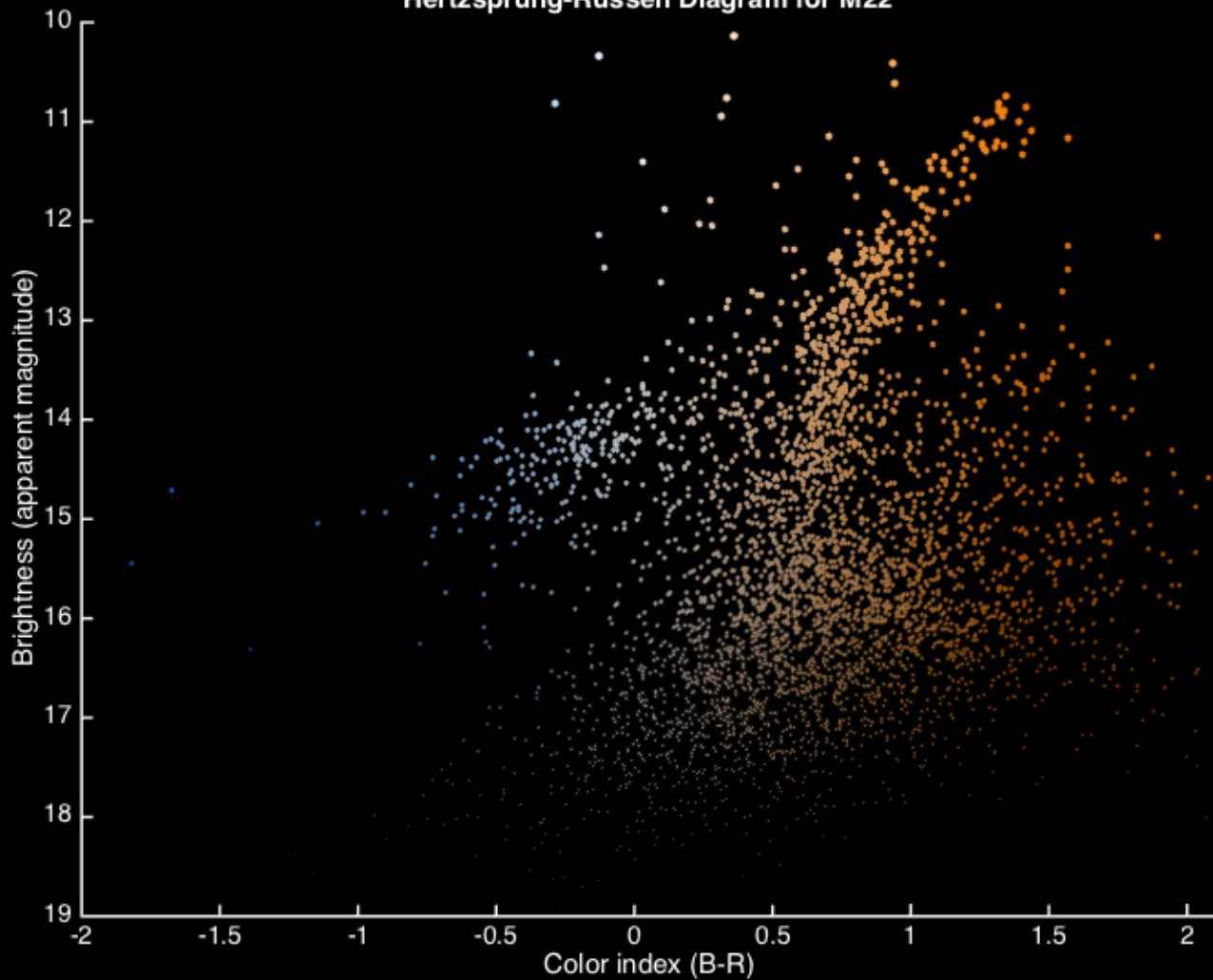
Hertzsprung-Russell Diagram for M22
