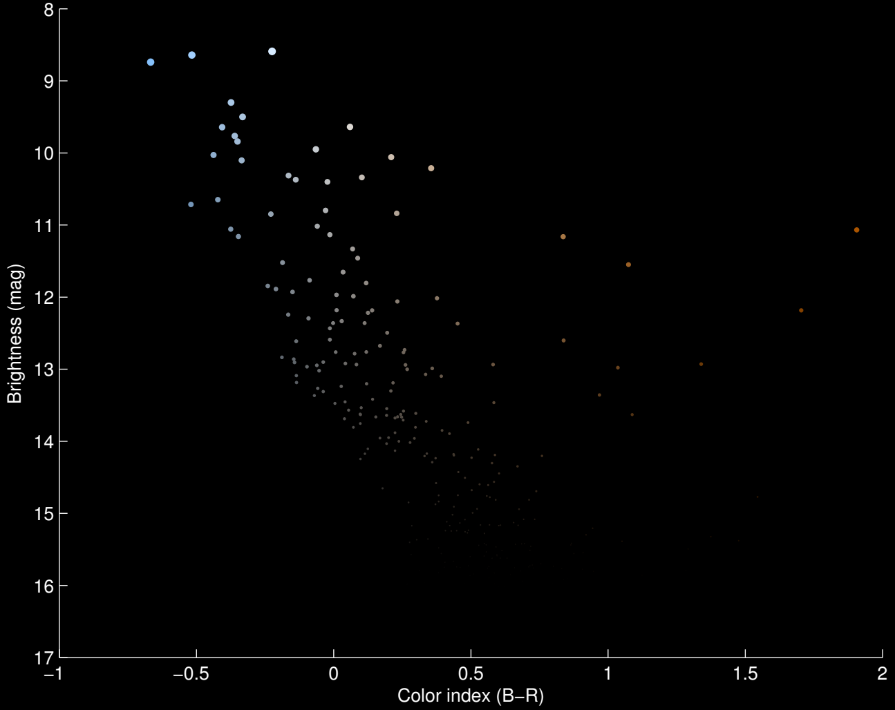
Hertzprung–Russell Diagram for M29
