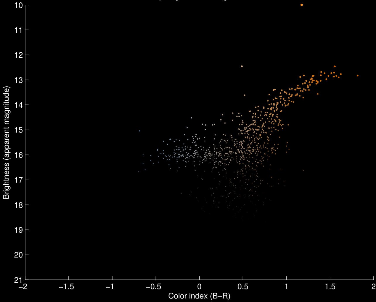
Hertzprung–Russell Diagram for M3
