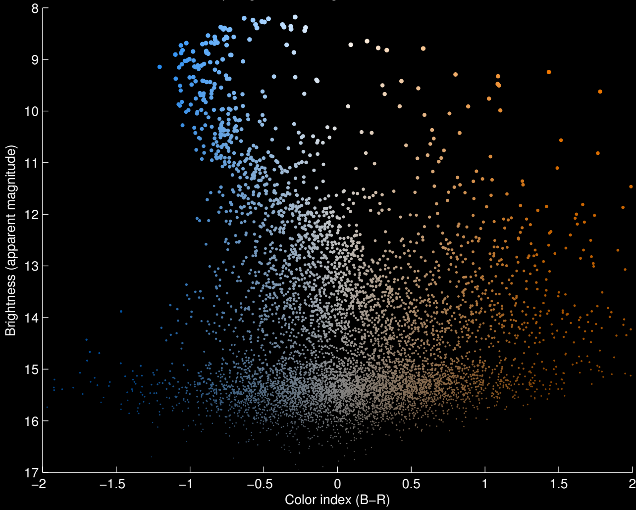
Hertzsprung–Russell Diagram for M35 and NGC2158
