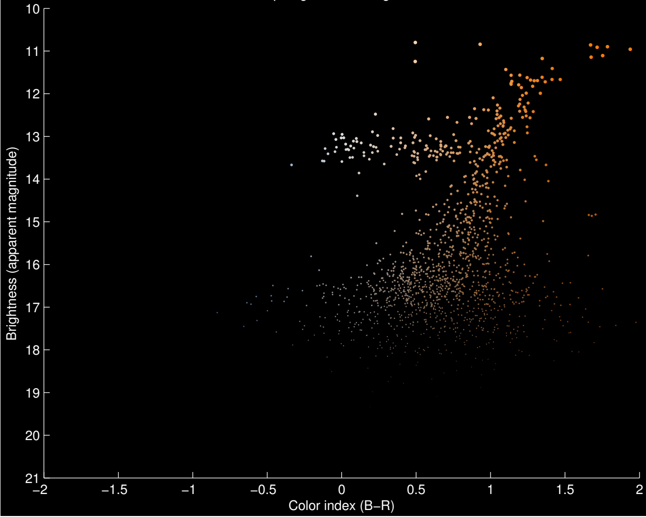
Hertzsprung–Russell Diagram for M4
