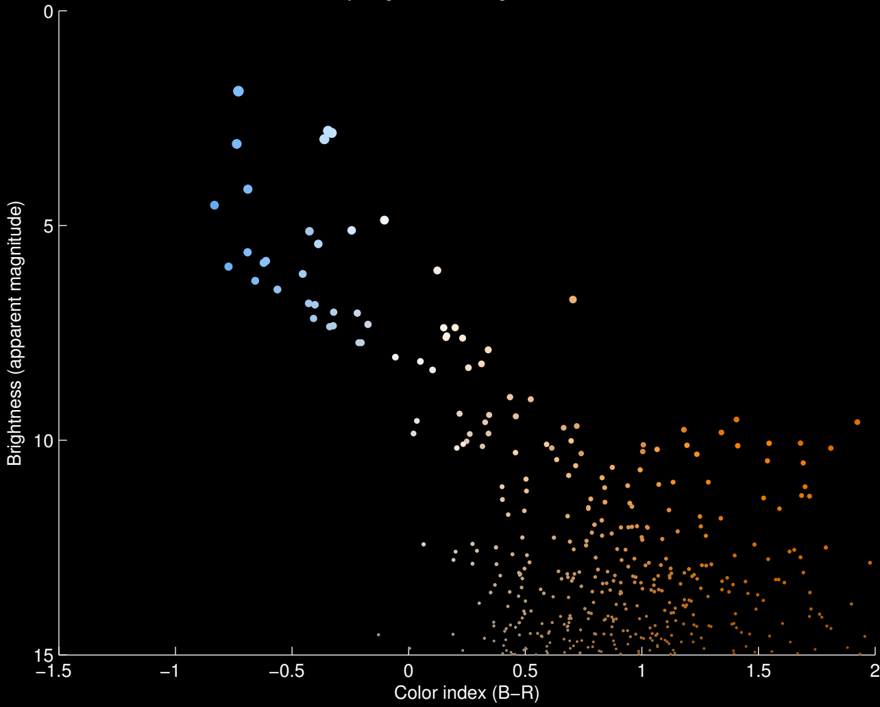
Hertzprung–Russell Diagram for M45–blur
