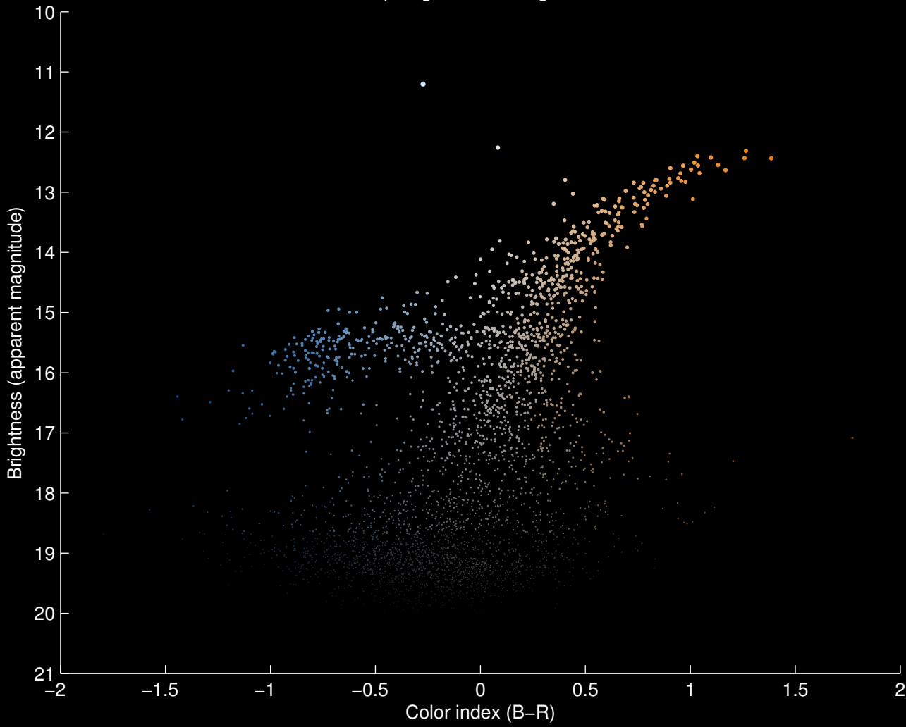
Hertzprung–Russell Diagram for M5
