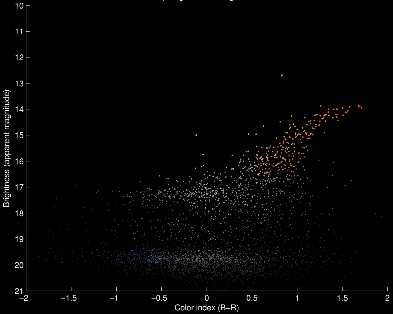
Hertzprung–Russell Diagram for M53
