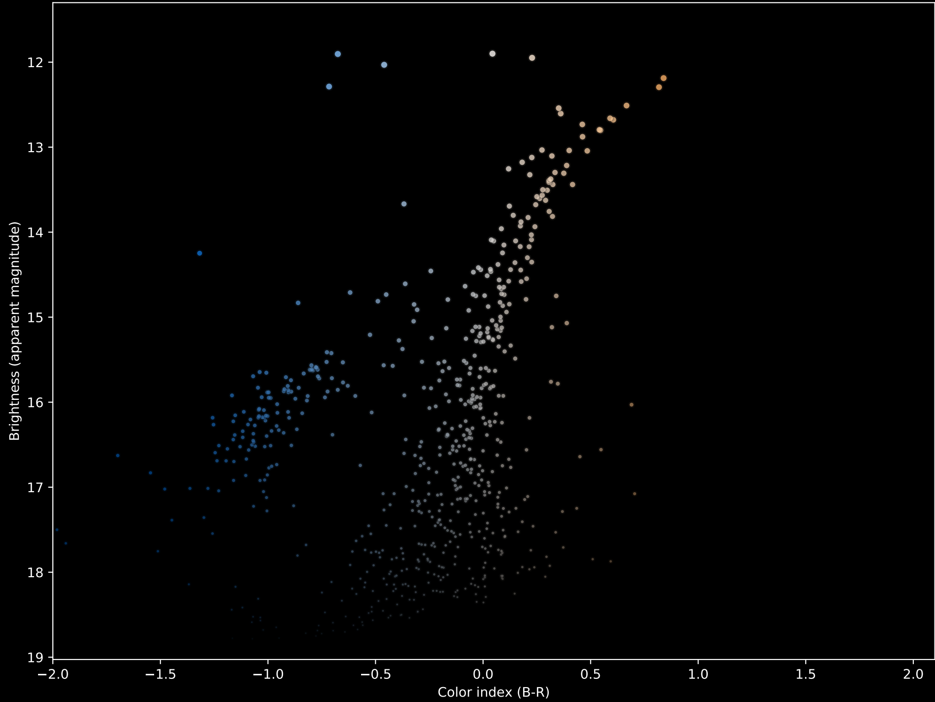
Hertzprung-Russell Diagram for M56
