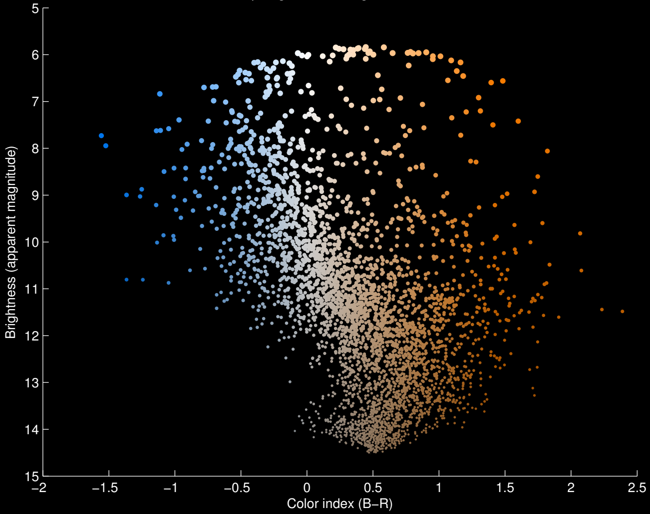
Hertzsprung–Russell Diagram for NGC2237
