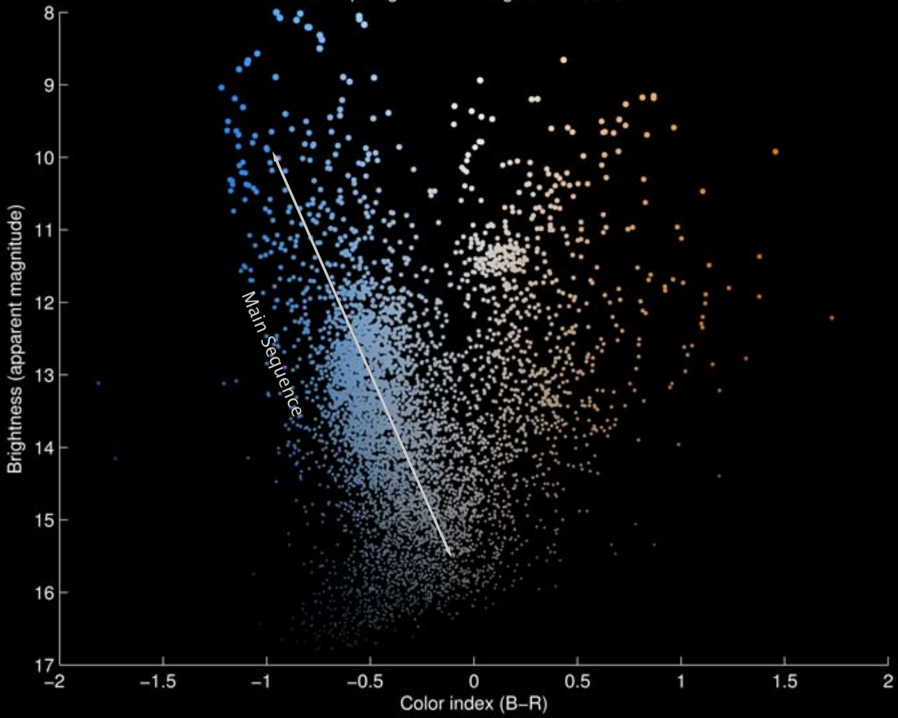
Hertzprung–Russell Diagram for NGC7789
