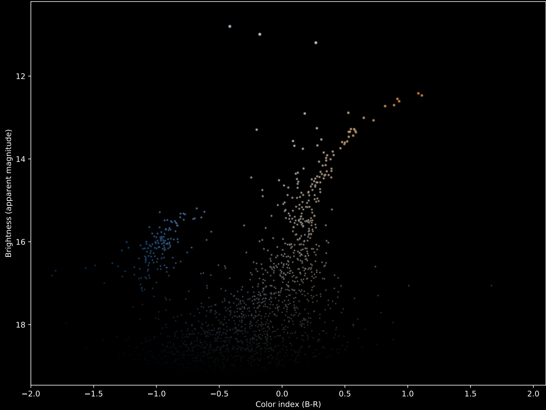
Hertzsprung-Russell Diagram for M12
