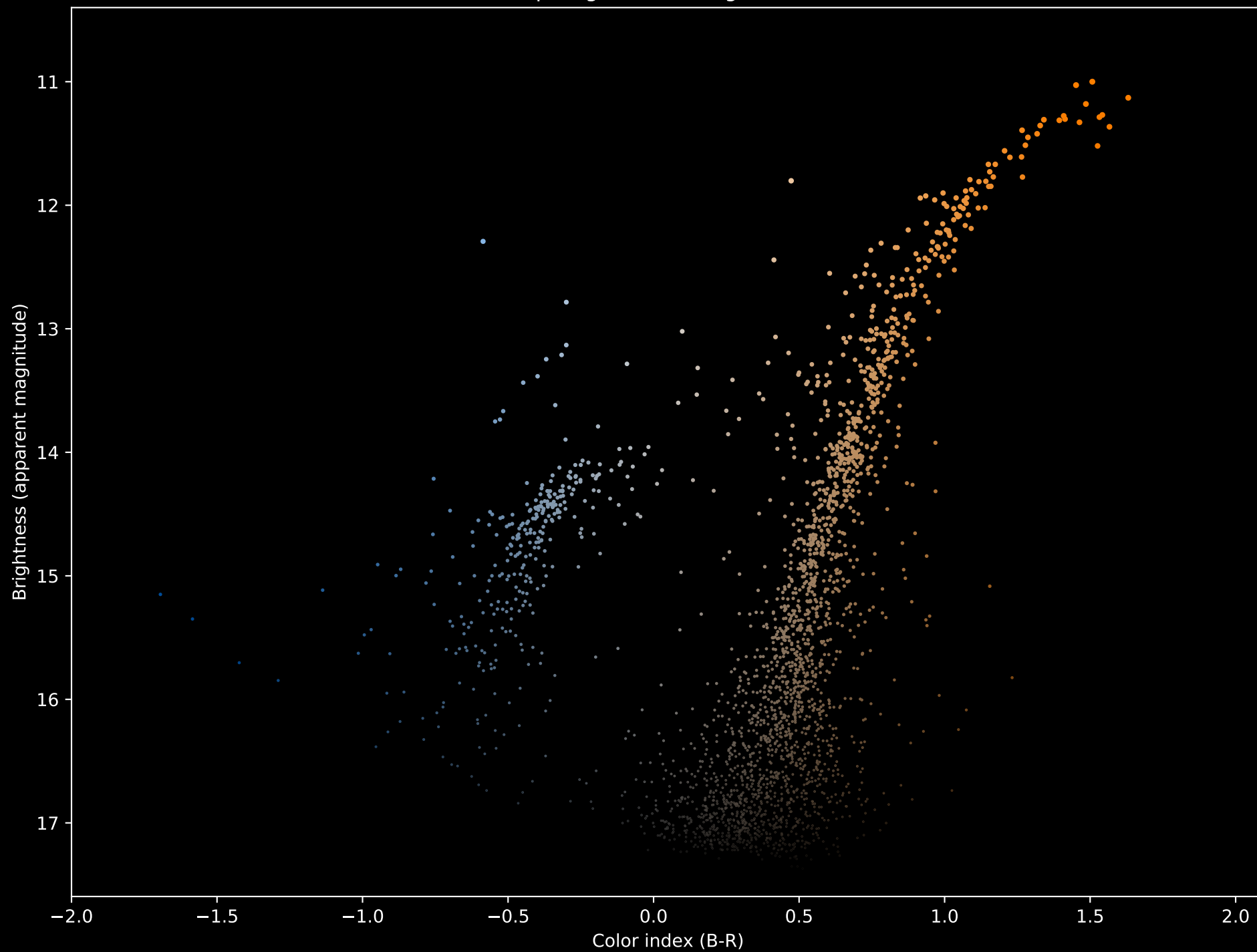
Hertzsprung-Russell Diagram for M13
