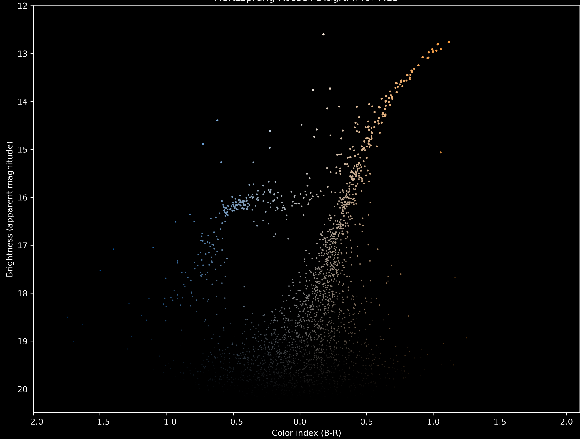
Hertzprung-Russell Diagram for M15
