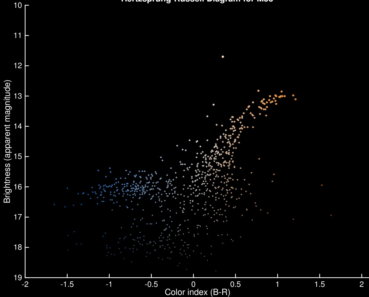
Hertzprung-Russell Diagram for M53
