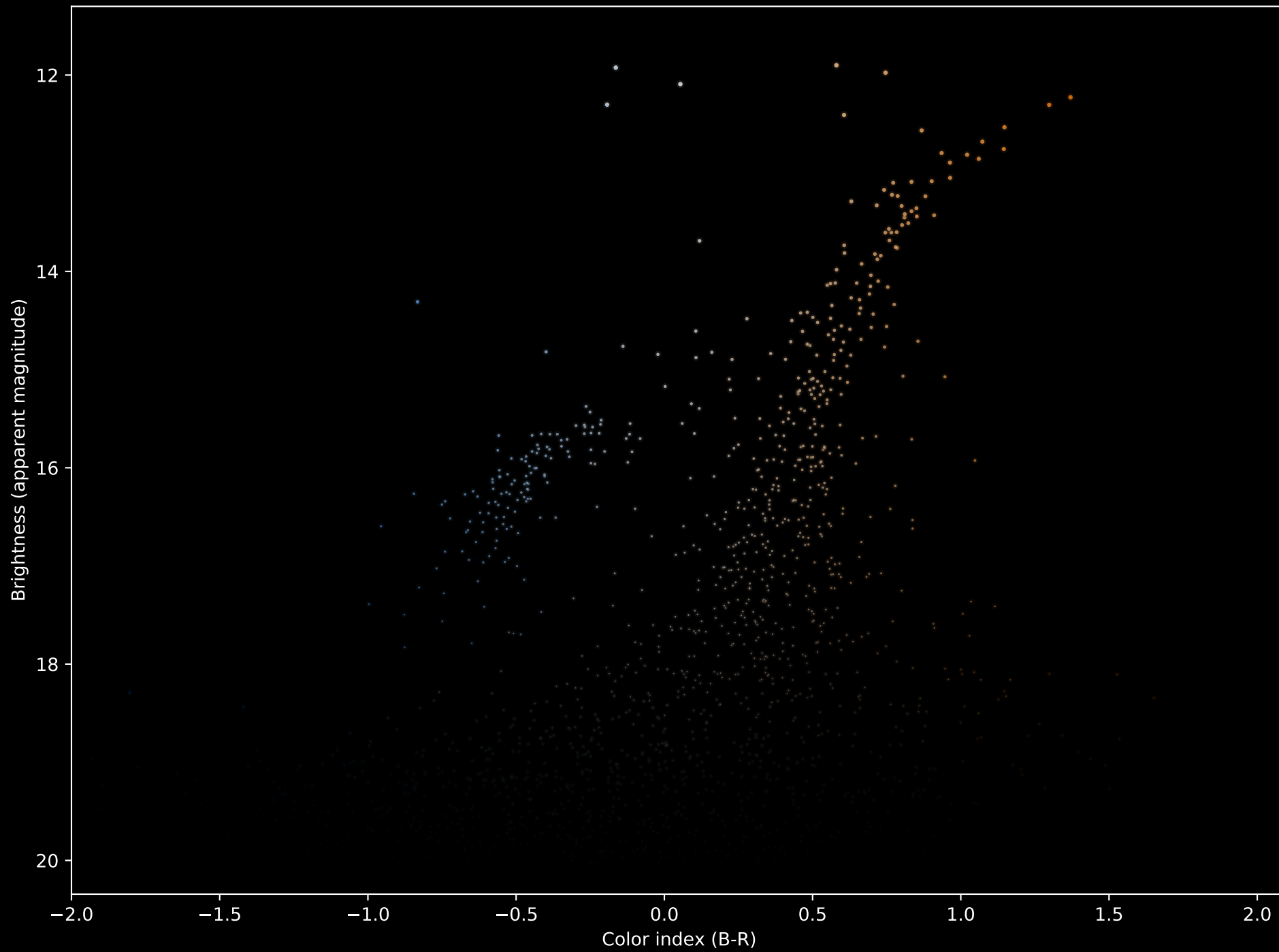
Hertzsprung-Russell Diagram for M56
