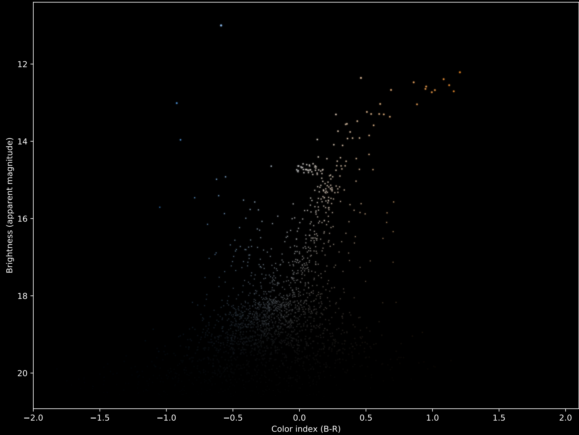
Hertzsprung-Russell Diagram for M71
