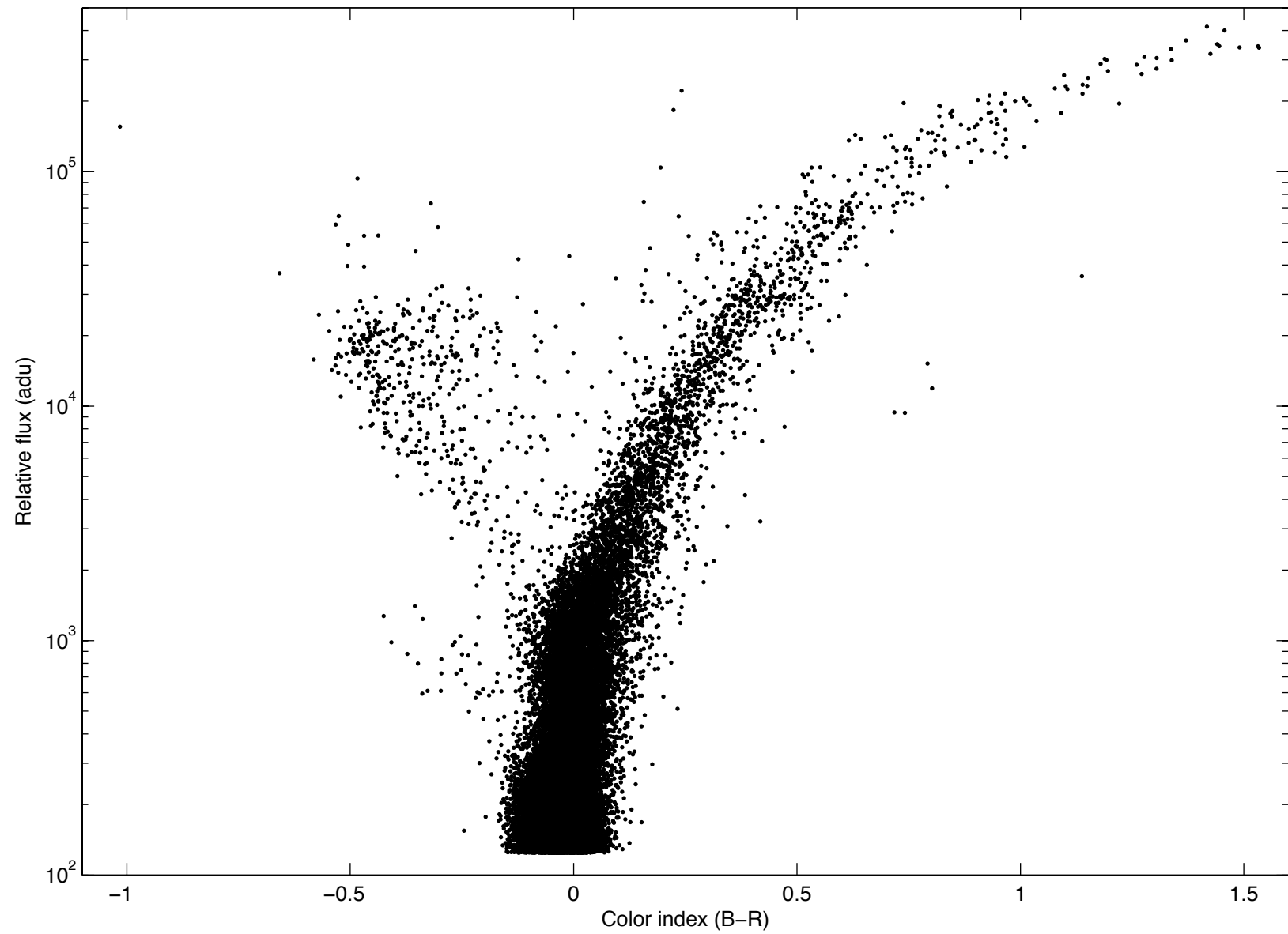
Hertzsprung–Russell Diagram for M13
