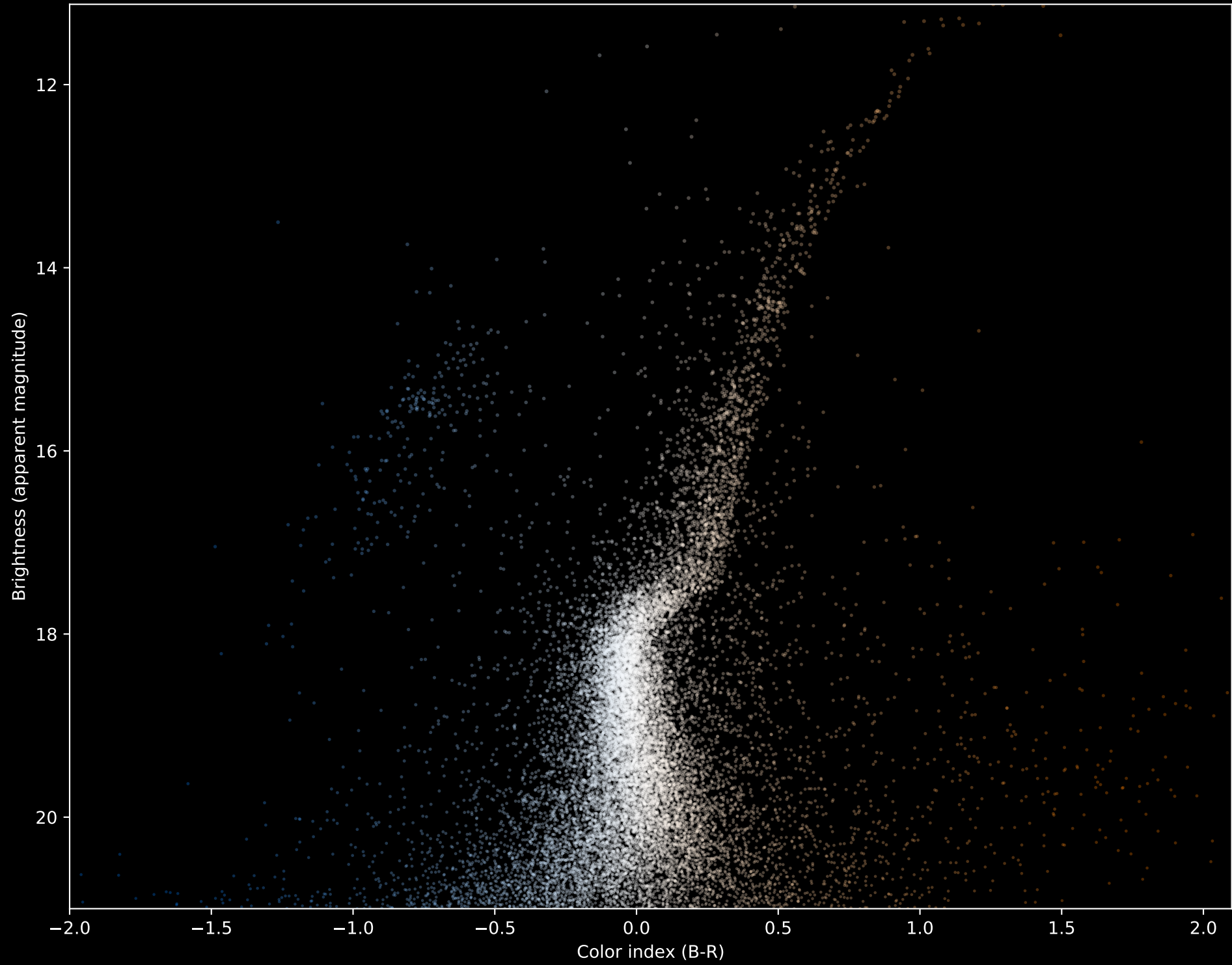
M10 Hertzprung-Russell Diagram using Gaia Data
