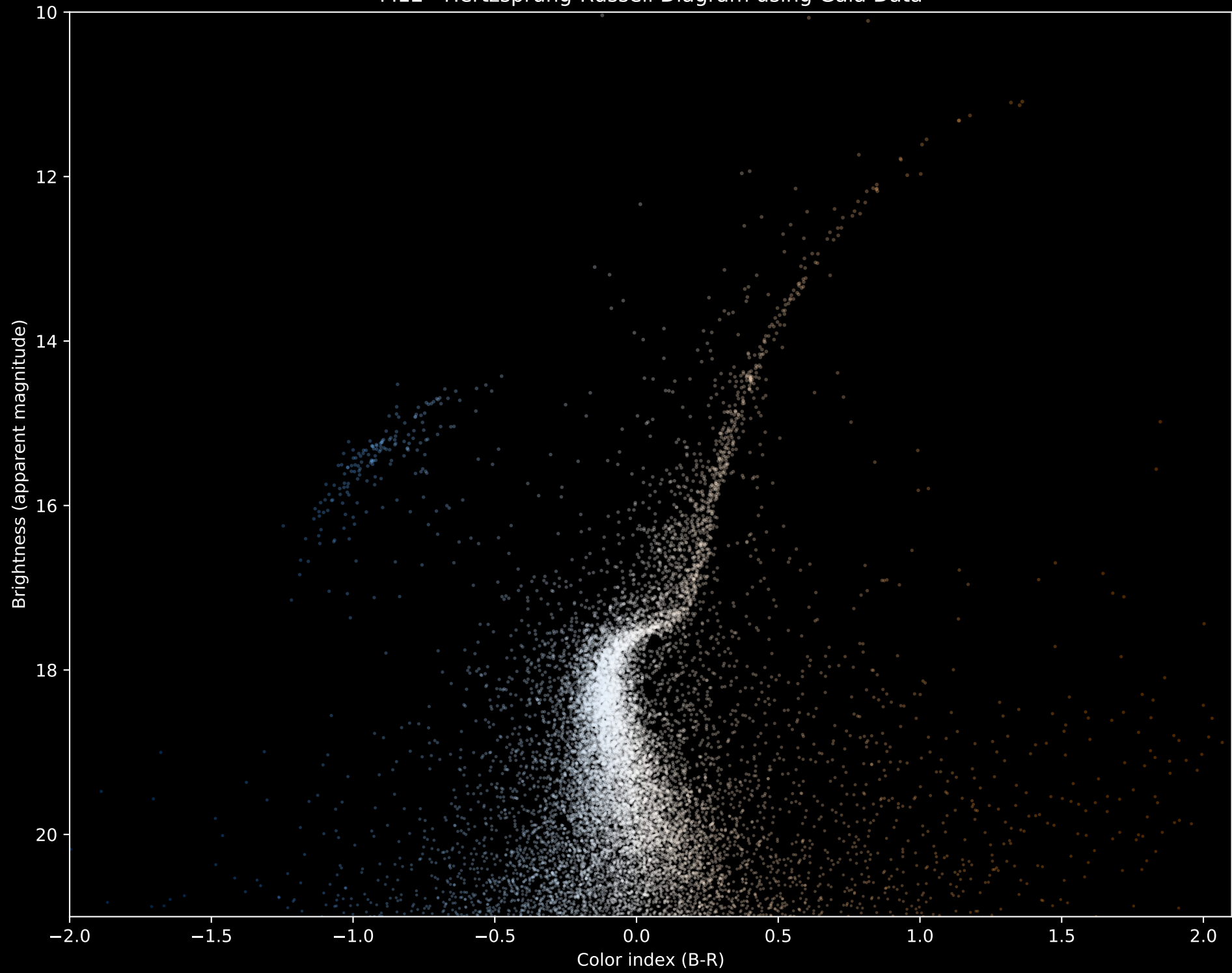
M12 Hertzprung-Russell Diagram using Gaia Data
