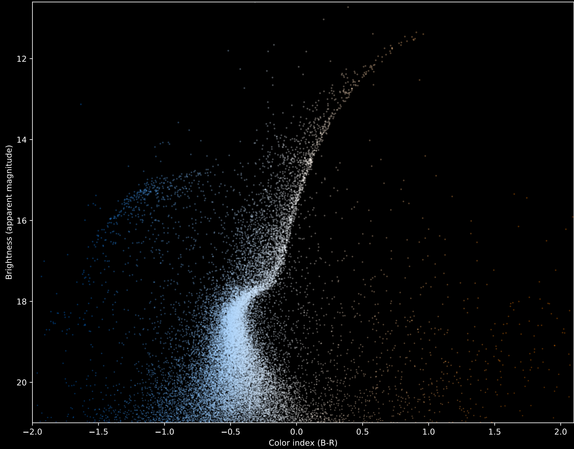
M13 Hertzprung-Russell Diagram using Gaia Data
