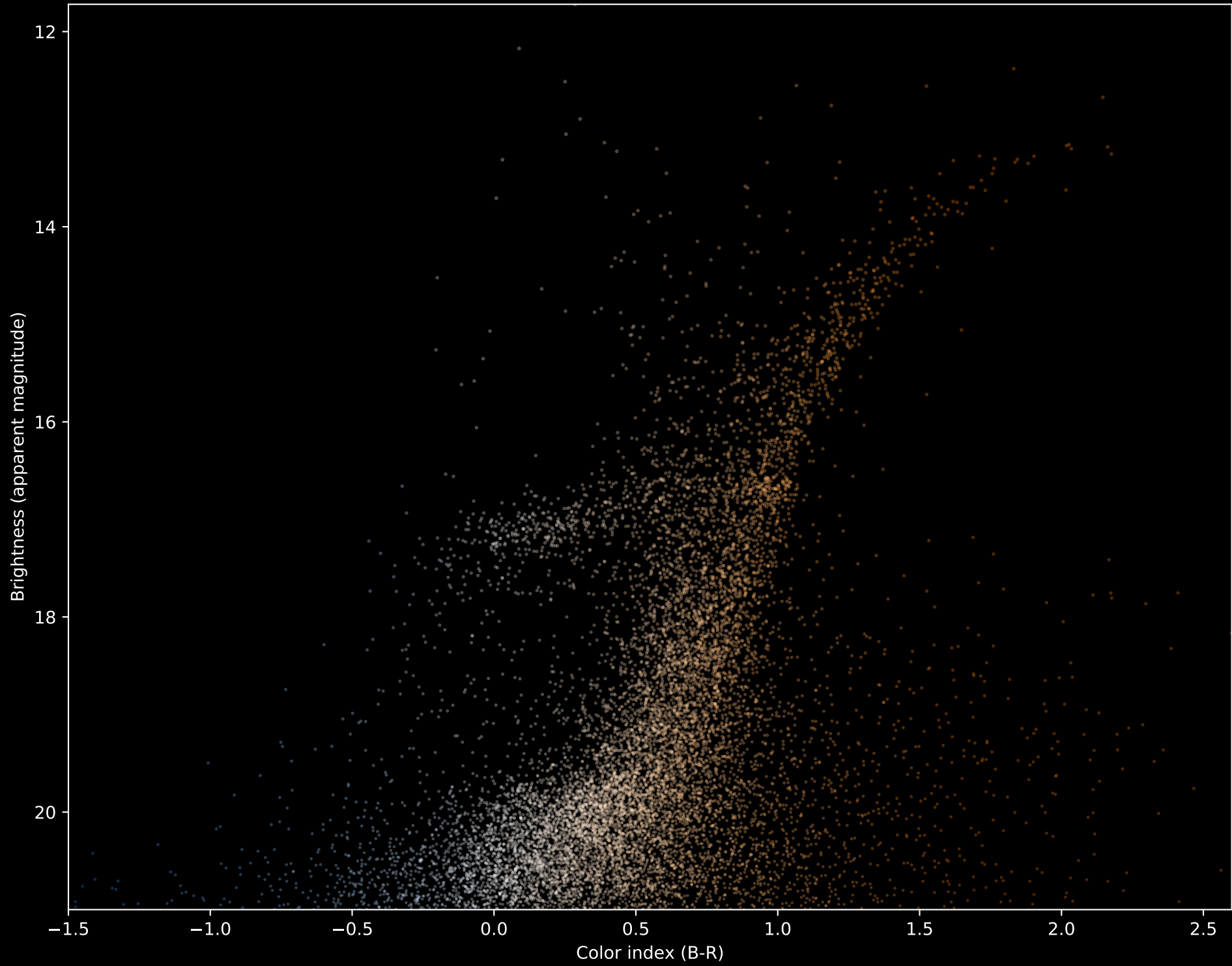
M14 Hertzprung-Russell Diagram using Gaia Data
