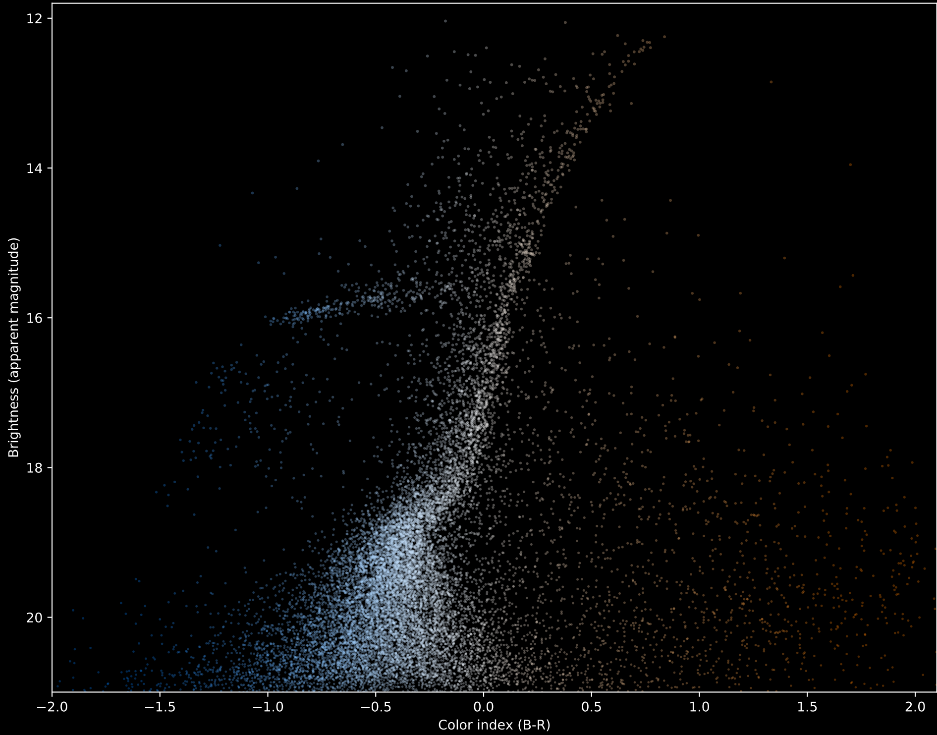
M15 Hertzprung-Russell Diagram using Gaia Data
