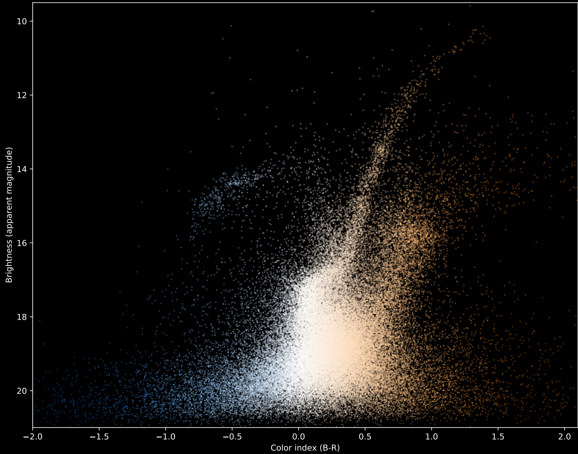
M22 Hertzprung-Russell Diagram using Gaia Data
