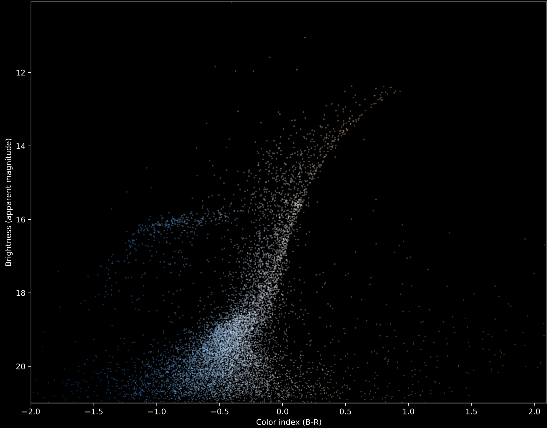
M2 Hertzprung-Russell Diagram using Gaia Data
