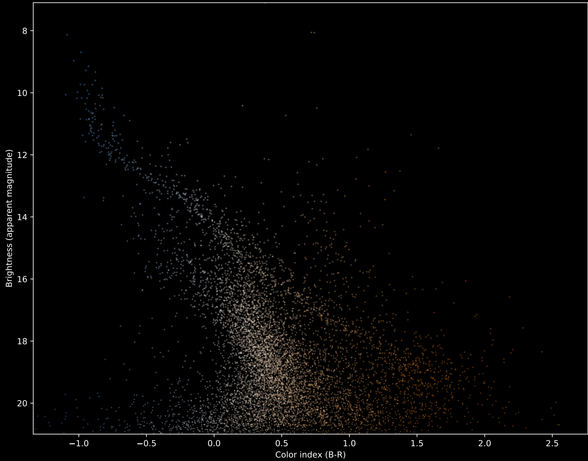
M35 Hertzprung-Russell Diagram using Gaia Data
