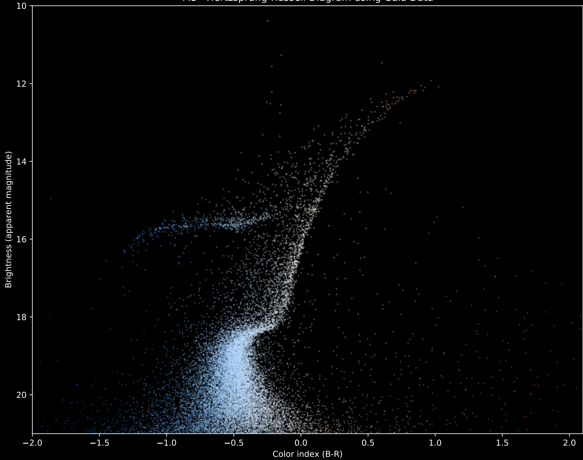
M3 Hertzprung-Russell Diagram using Gaia Data
