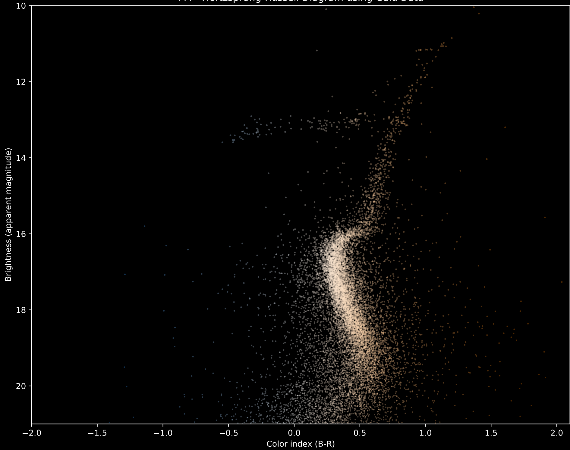
M4 Hertzprung-Russell Diagram using Gaia Data
