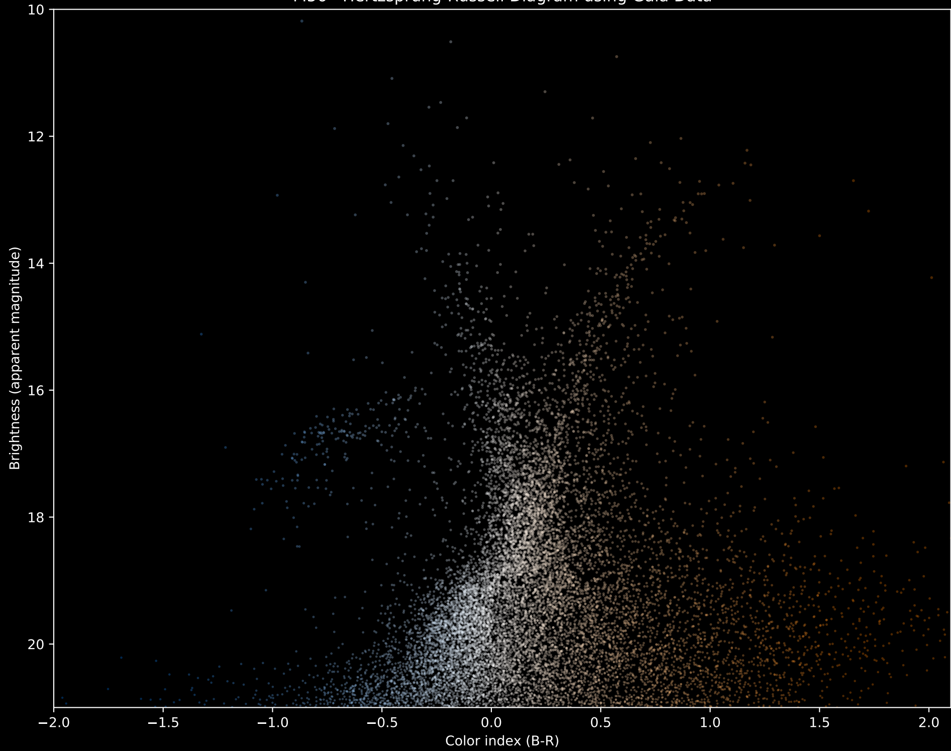
M56 Hertzprung-Russell Diagram using Gaia Data
