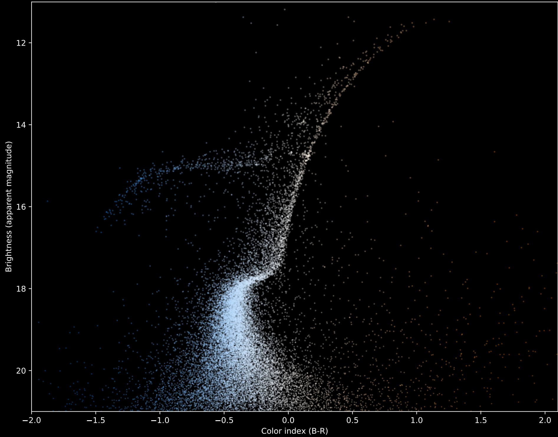
M5 Hertzprung-Russell Diagram using Gaia Data
