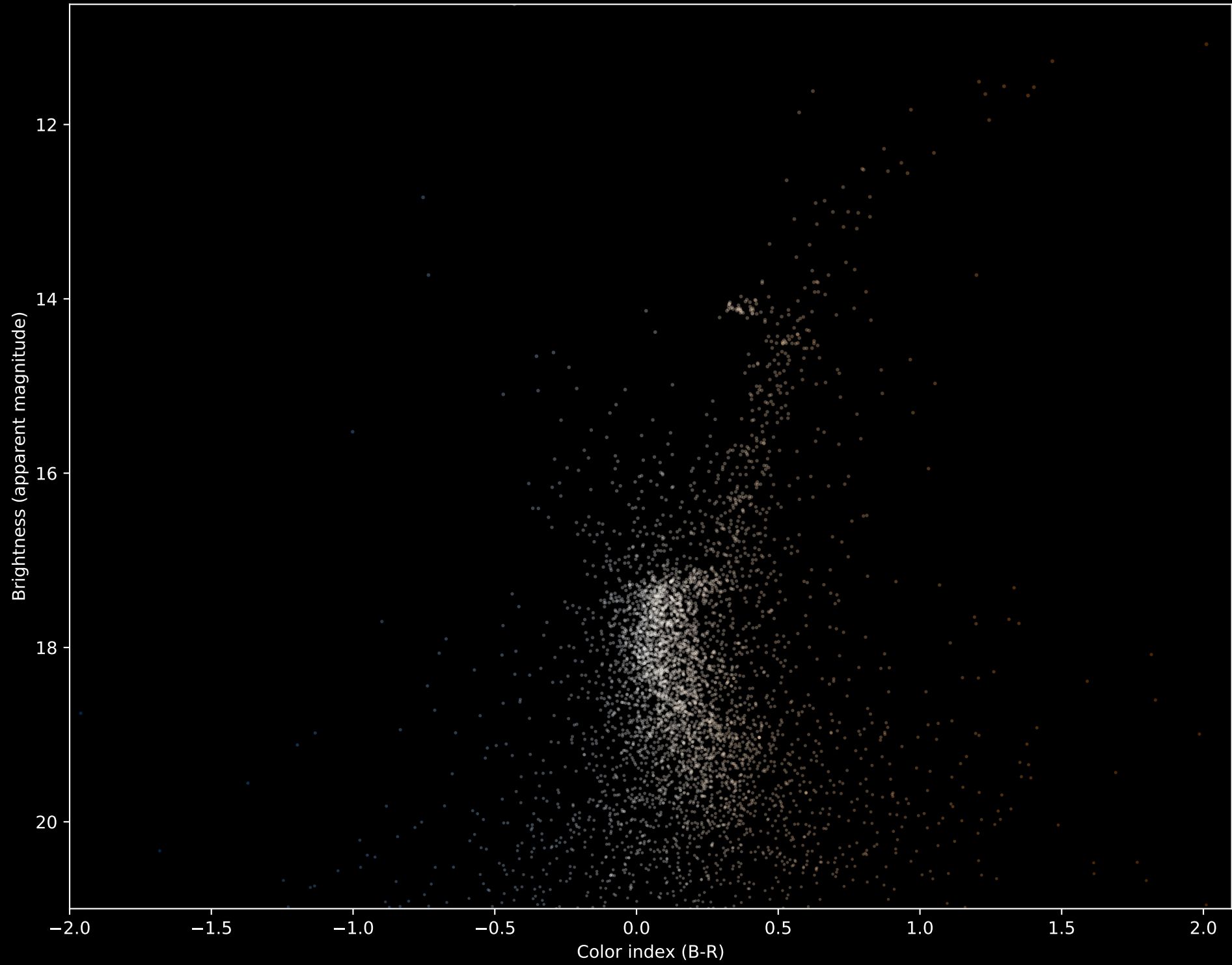
M71 Hertzprung-Russell Diagram using Gaia Data
