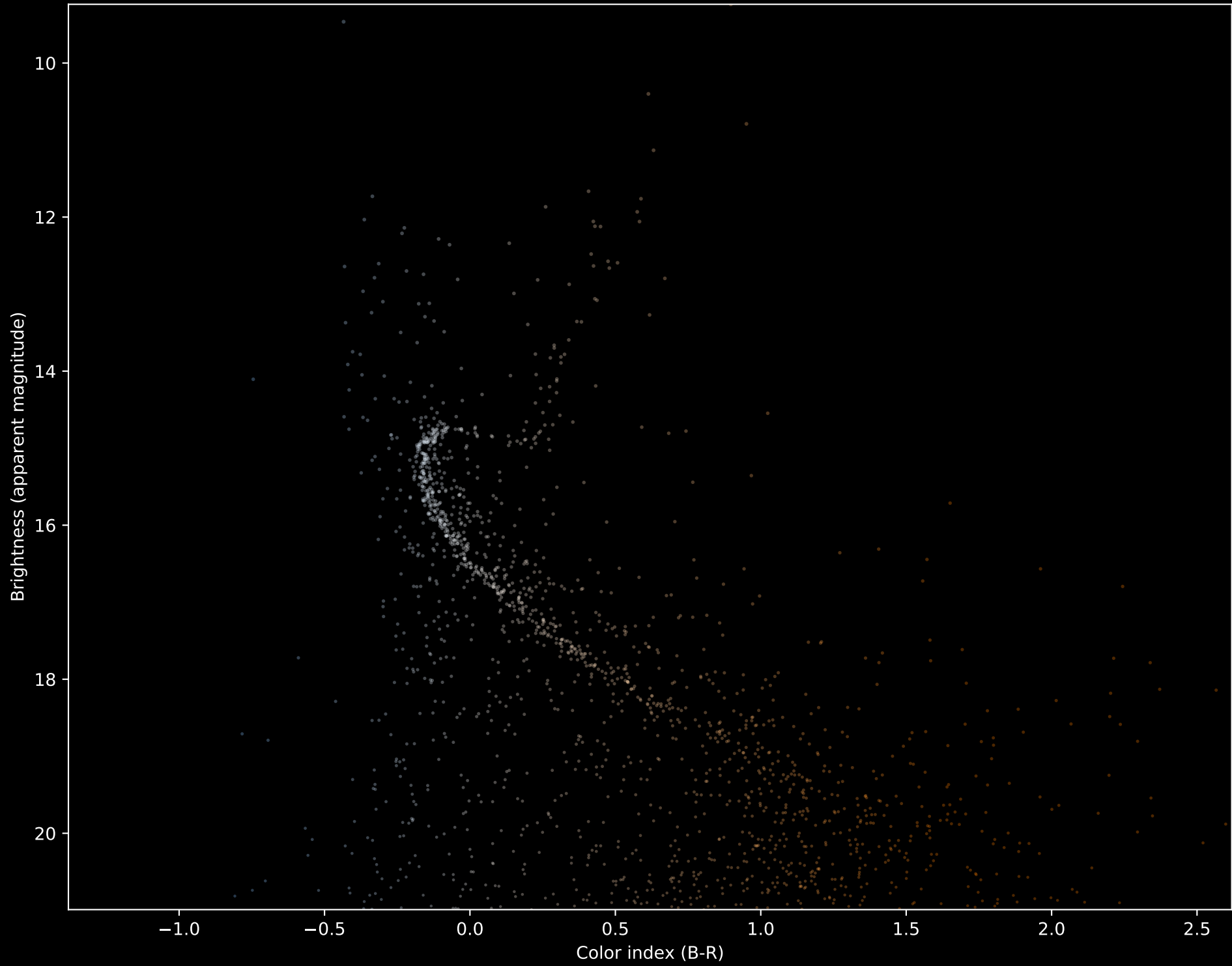
NGC 188 Hertzprung-Russell Diagram using Gaia Data
