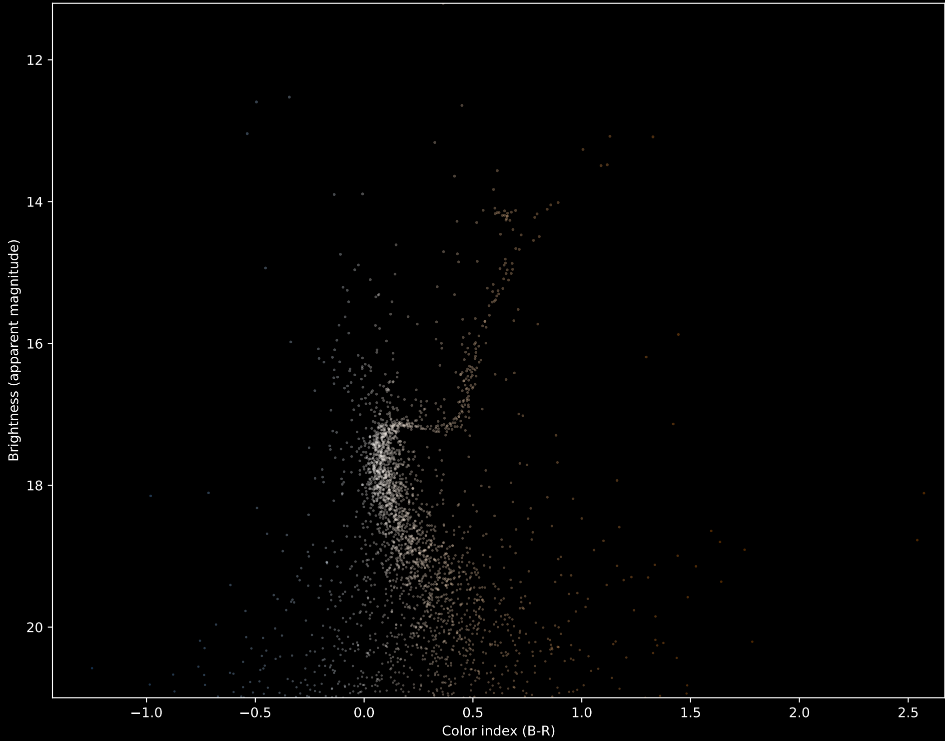
NGC 6791 Hertzprung-Russell Diagram using Gaia Data
