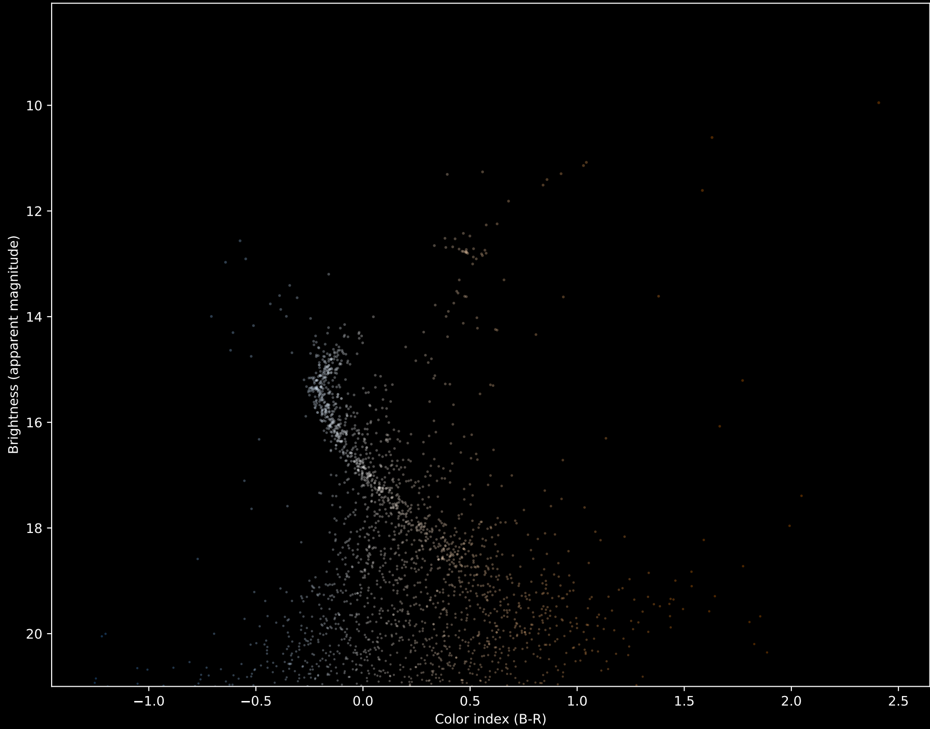
NGC 6819 Hertzsprung-Russell Diagram using Gaia Data
