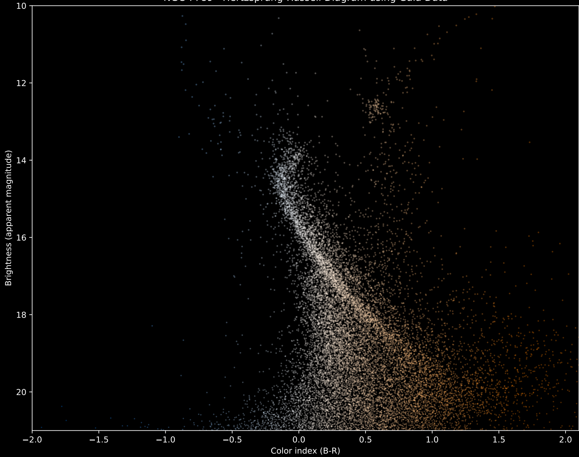
NGC 7789 Hertzsprung-Russell Diagram using Gaia Data
