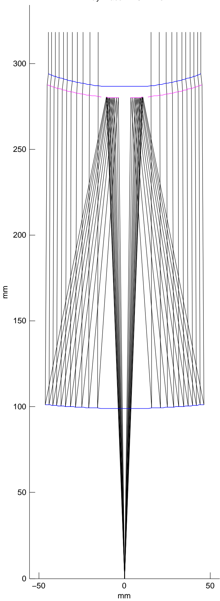
Ray Trace -- On Axis
