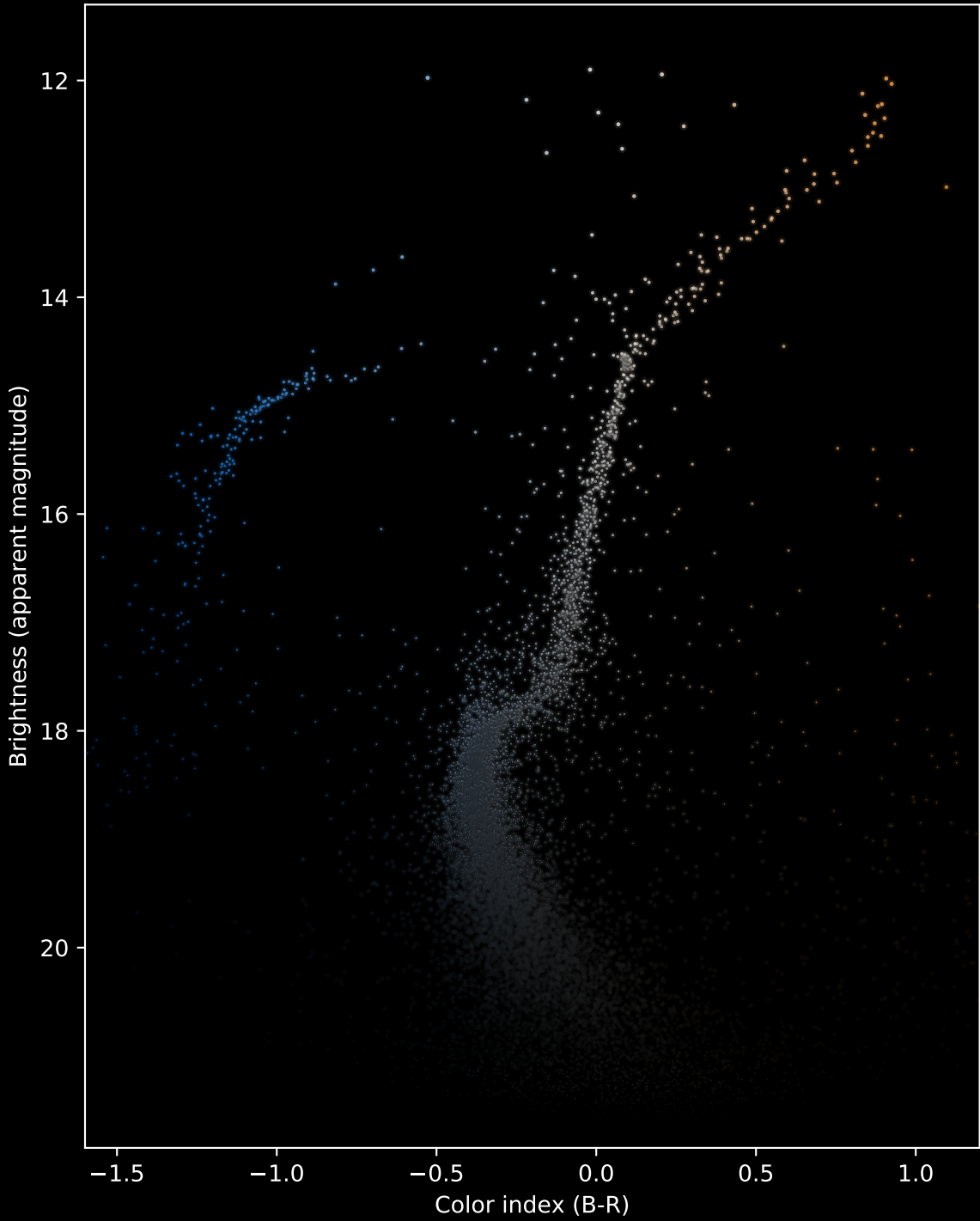
Hertzsprung-Russell Diagram for M13
