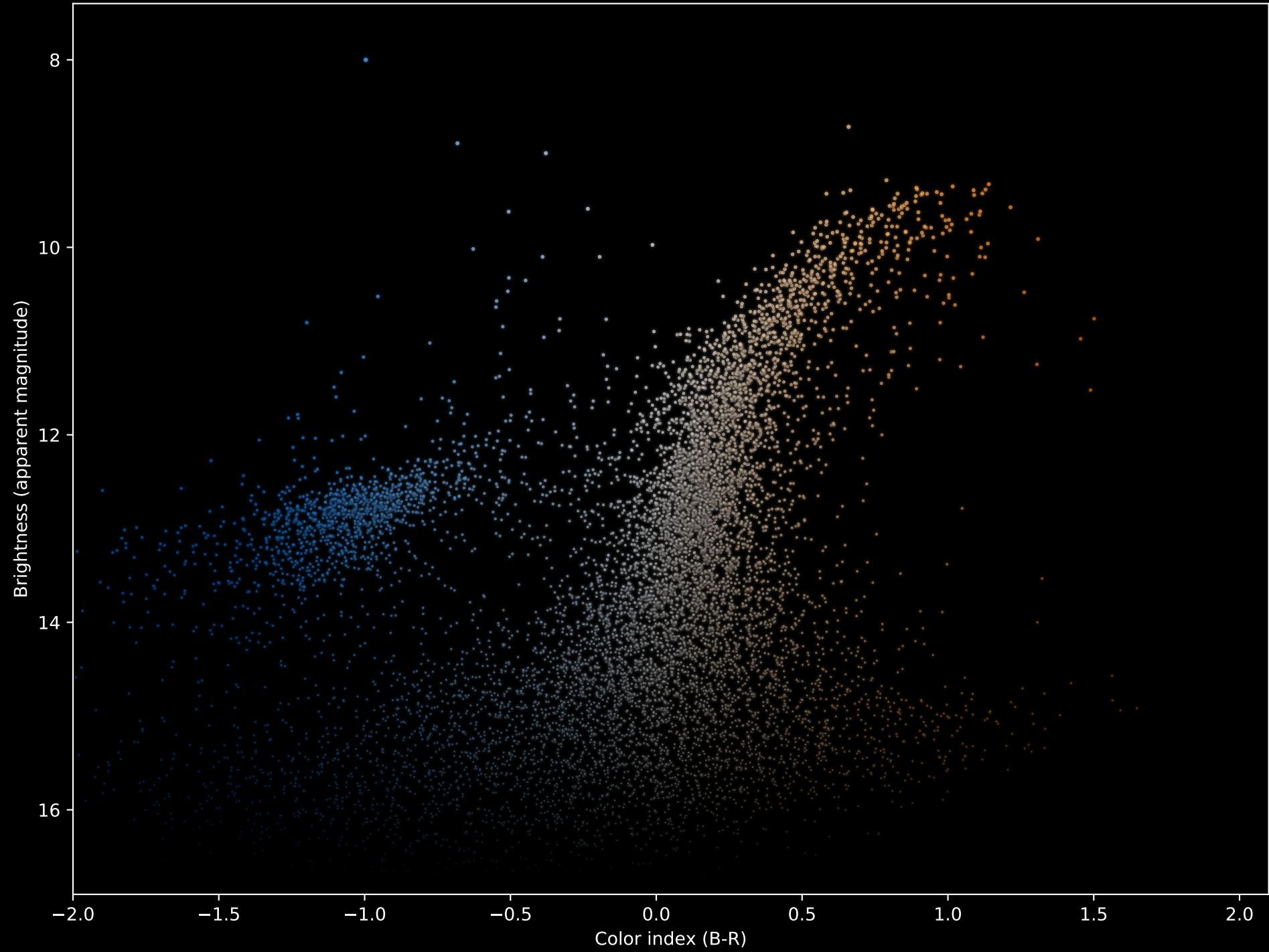
Hertzsprung-Russell Diagram for OmegaCentauri
