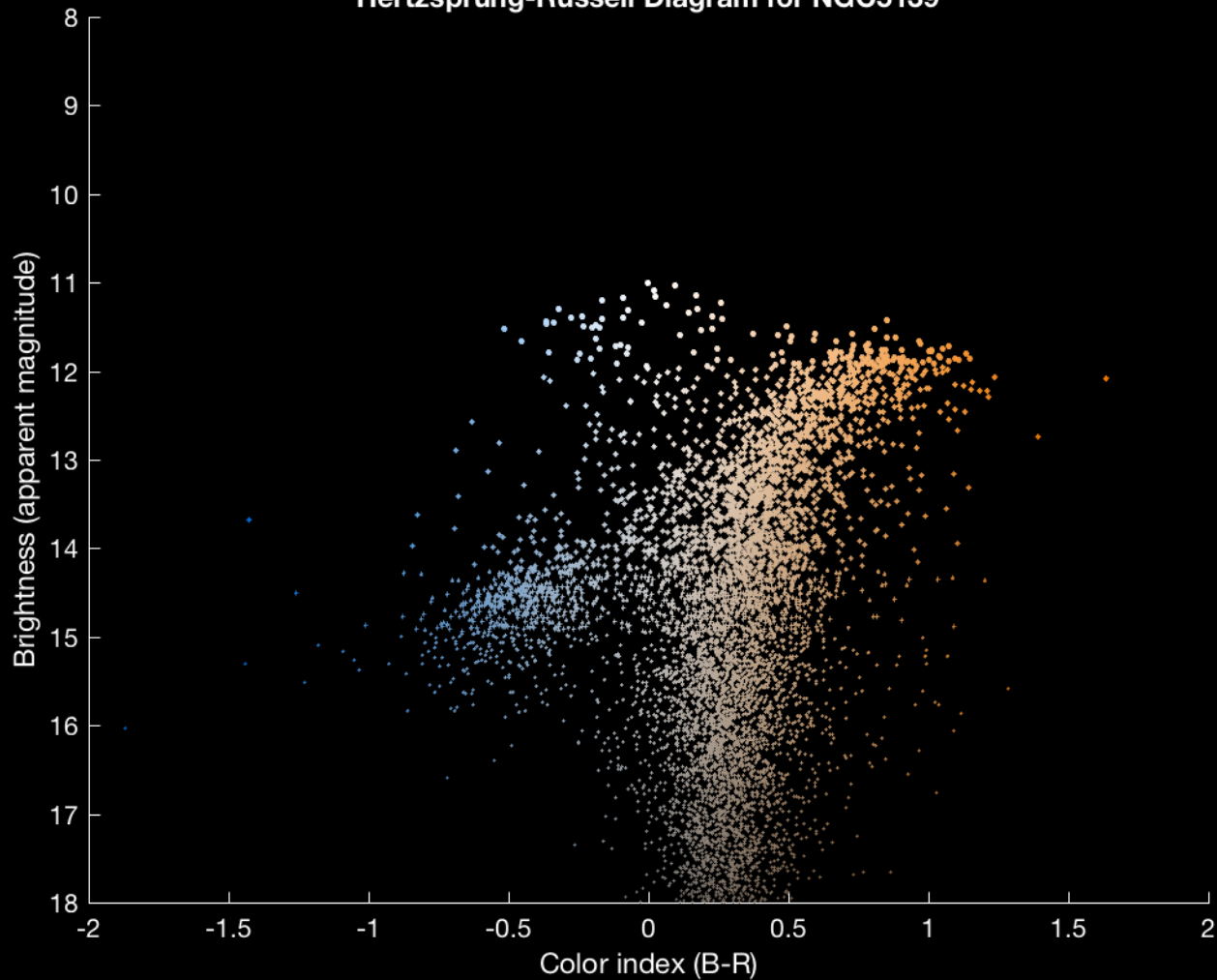
Hertzprung-Russell Diagram for NGC5139
